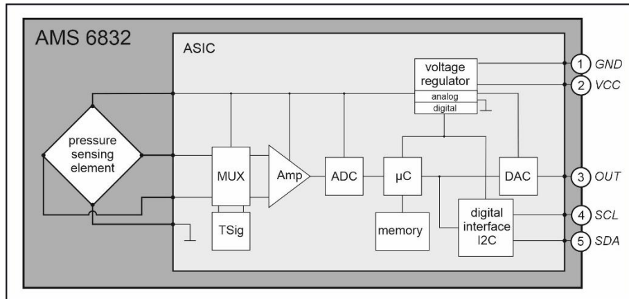
Figure 1: Functional principle
